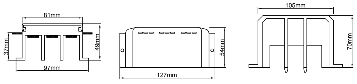
Busbar Type 0 125A
