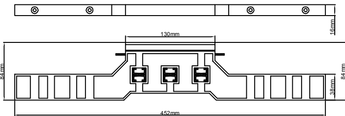
Busbar Type 4 400A
