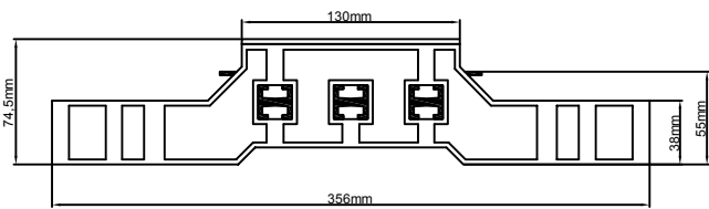
Busbar Type 1 400A
