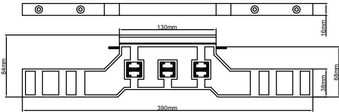
Busbar Type 2 400A
