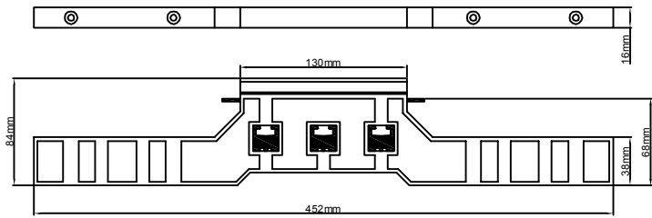
Busbar Type 4 800A
