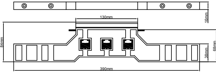
Busbar Type 2 800A
