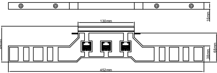
Busbar Type 3 800A
