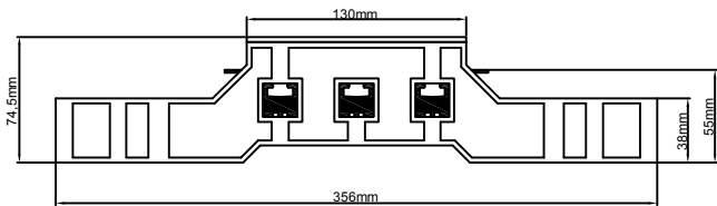
Busbar Type 1 800A
